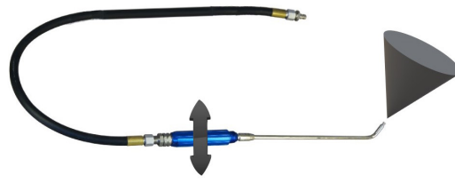
Air extension wand Deluxe 10" wand with 45° hook with conical spray pattern 18" hose, handle with swivel.
