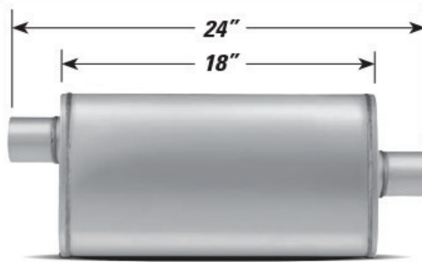
OFFSET/CENTER (4" x 9")
