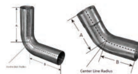
Elbows
