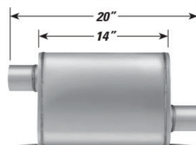
OFFSET/OFFSET (4" x 9")
